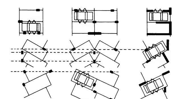
④ Possible positions of columns
